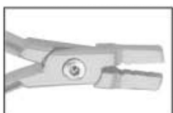
A-DTL-3186 For double back and triple back bands in 0.30" / .76mm & 0.36 / .91mm lingual arch wires.
