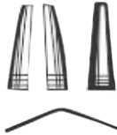
A-DTL-3169 Aderer Clamp three jaw Wire bending plier for contouring and Bending wire up to .30"/.76 mm
